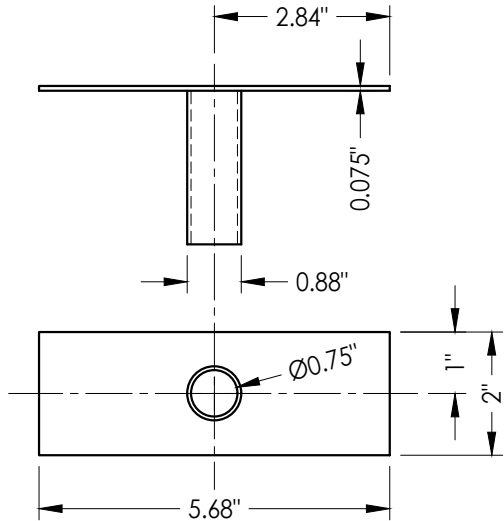
9 TUBE ANCHOR
